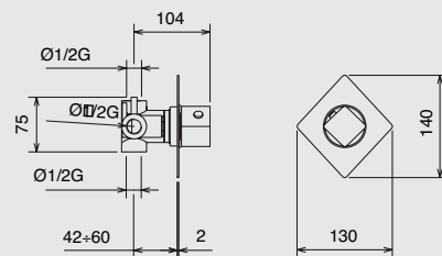
19955 thermostat
