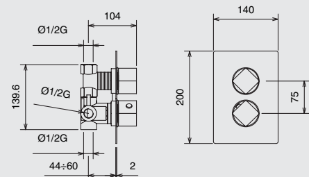
19950 thermostat
